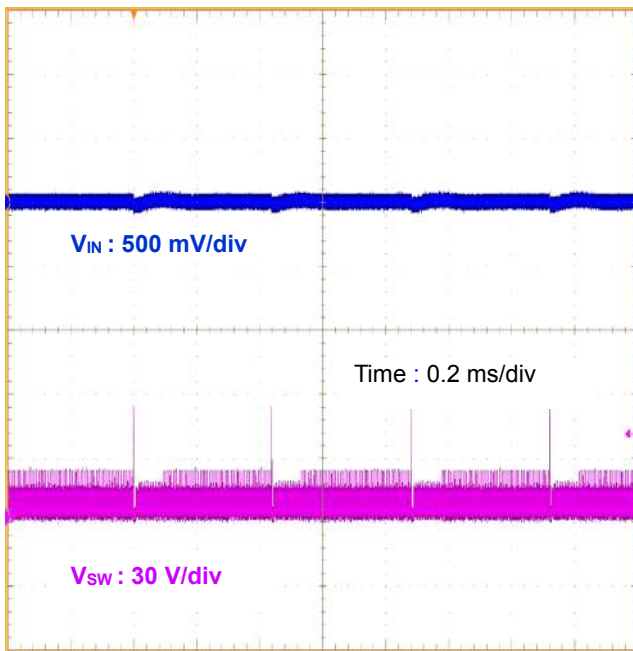
Figure 21. V_{IN} リップル波形 ( V_{IN} = 48\text{ V} , V_{OUT} = 5\text{ V} , f_{OSC} = 200\text{ kHz} , I_{OUT} = 0\text{ A} )
