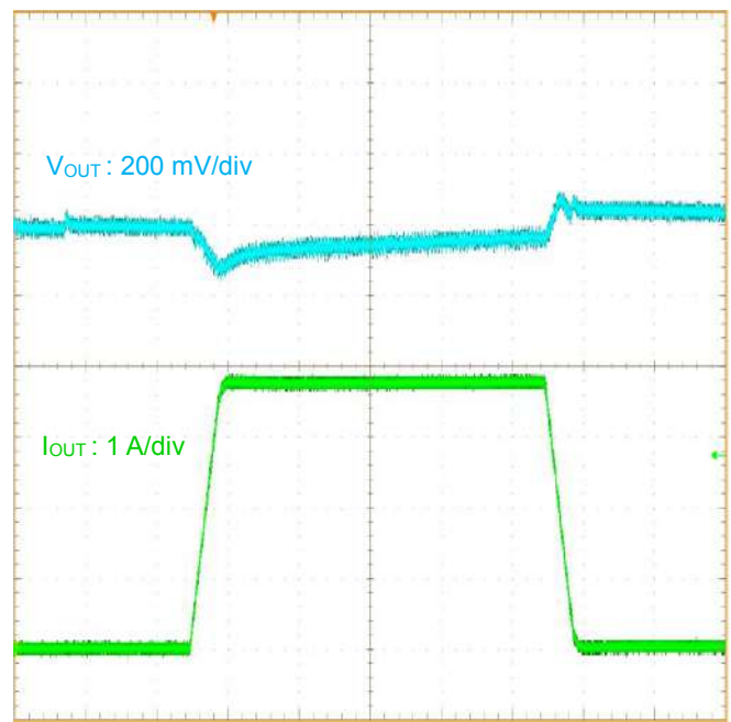
Figure 42. Load Transient Response ( I_{OUT} = 0\text{ A} - 3.75\text{ A} )
